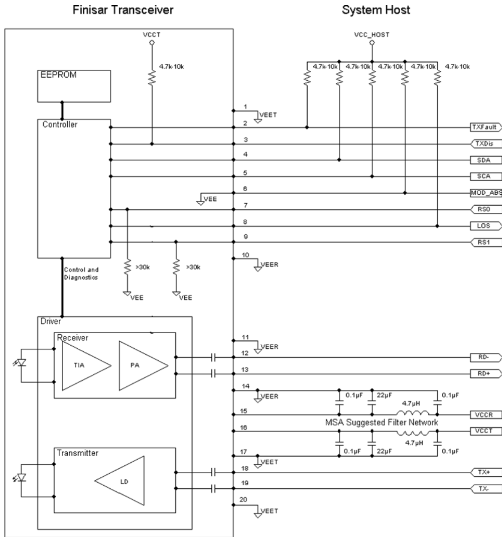
Figure 5. Host-Module Interface
