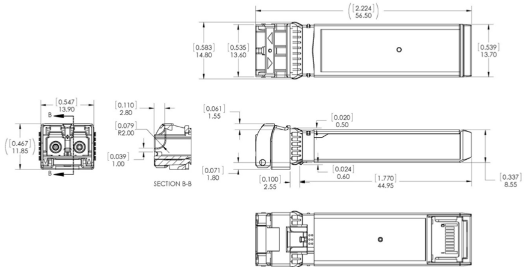
Figure 2. FTLX8574D3BNL Mechanical Dimensions and Tolerances.
