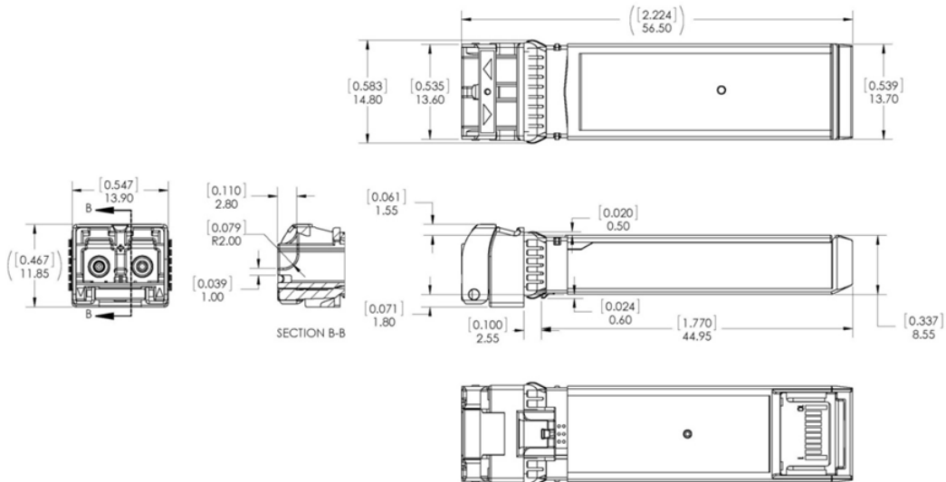
FTLF8532P4BNV
