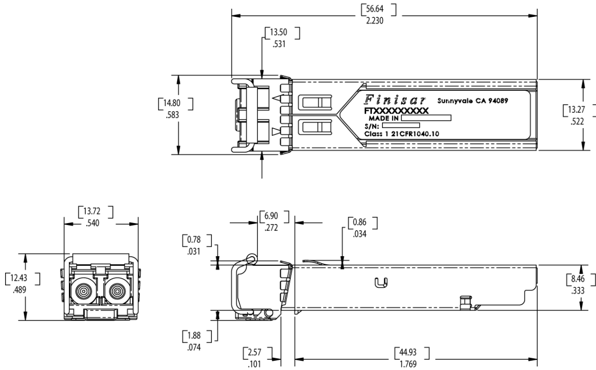
FTLF8524P2WNy
