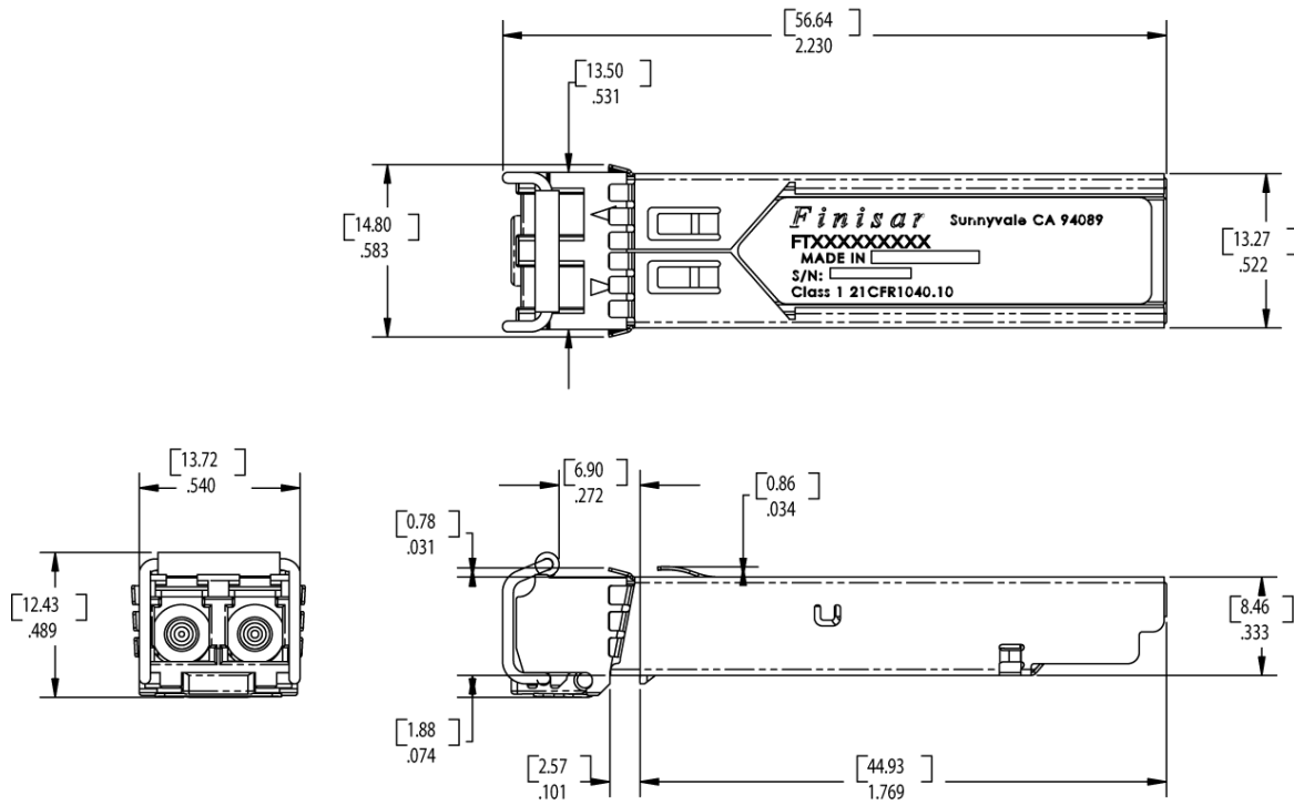
FTLF8524P2BNy
