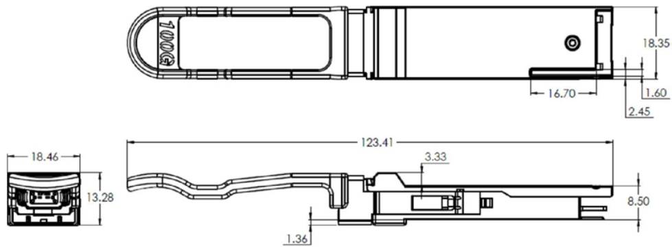
Figure 2. FTLC9558REPM Mechanical Dimensions.
