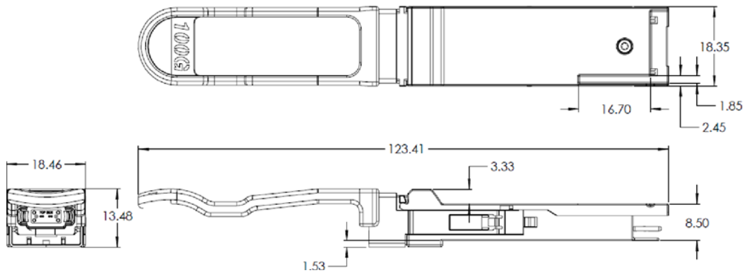
Figure 2. FTLC9555WEPM Mechanical Dimensions.
