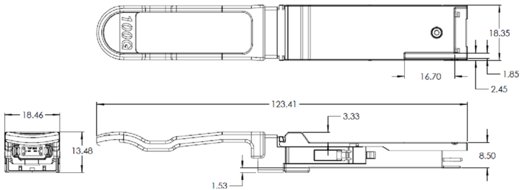
Figure 2. FTLC9152RGPL Mechanical Dimensions.
