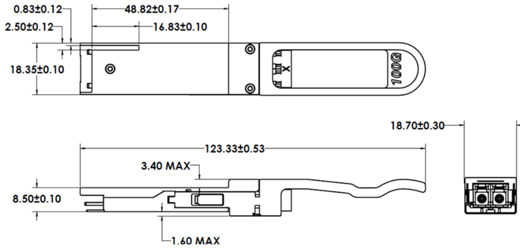
Figure 2. FTLC1155RGPLD Mechanical Dimensions.
