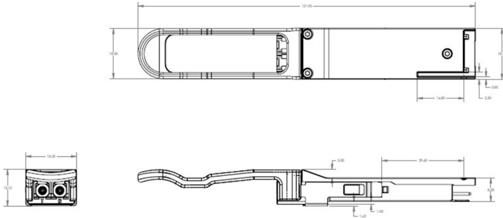
Figure 2 – FTL4E1QE1C mechanical drawing
