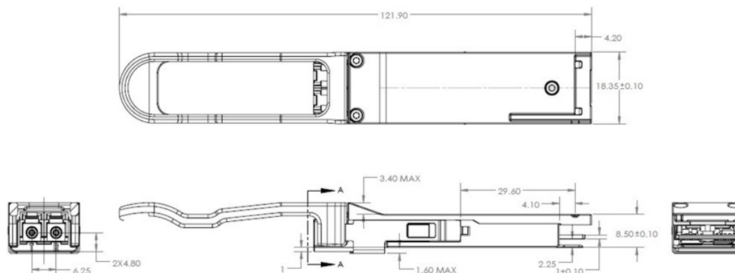
Figure 2 – FTL4C1QL2L mechanical drawing
