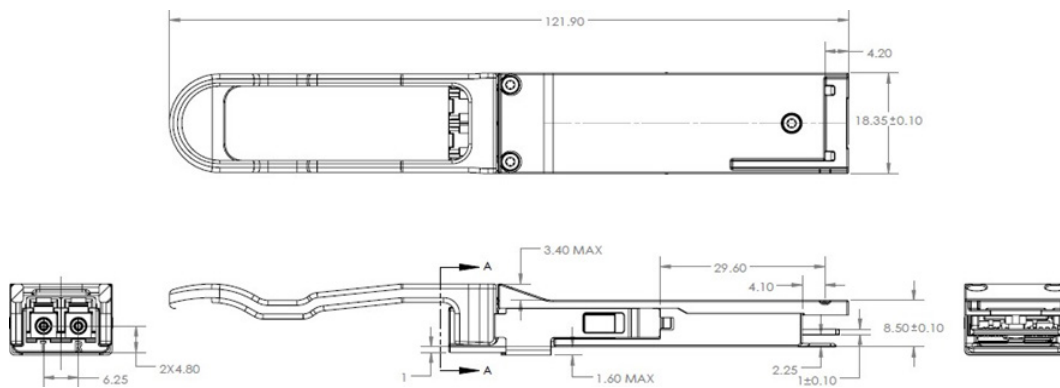
Figure 2 – FTL4C1QE3C mechanical drawing
