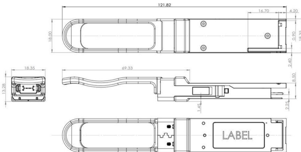
Figure 2 – FTL410QE4C mechanical drawing
