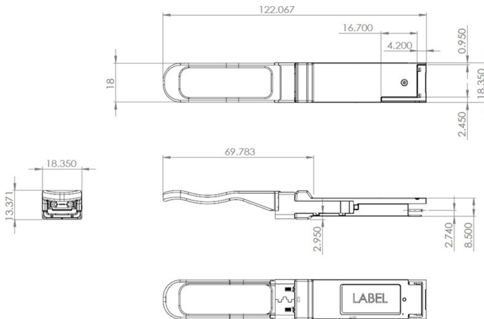
Figure 2 – FTL410QE3C mechanical drawing
