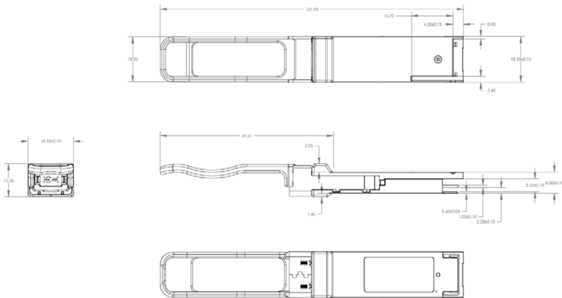
Figure 3 – FTL410QD2C mechanical drawing
