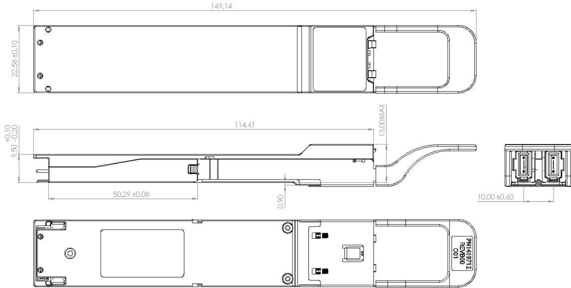
Figure 2. FTCE4527E1PxA-2N Mechanical Dimensions.
