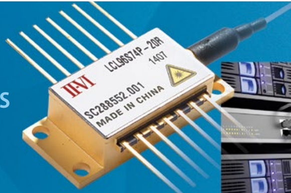
980nm Dual Chip Pump Laser Module
