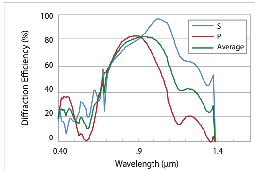
Typical absolute diffraction efficiency at AOI 61.2° *
